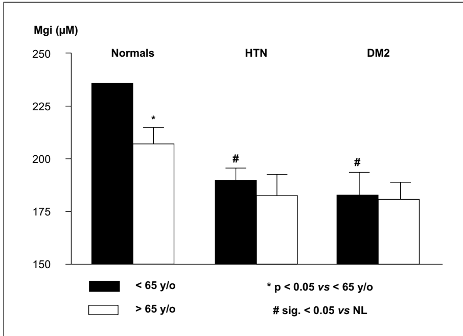
Figure 4. Effect of age on cytosolic free magnesium ( Mg_i ) levels in healthy normal, hypertensive (HTN) and in type 2 diabetic subjects (DM2) subjects (reproduced from [12] with permission). Full bars indicate data from young-middle aged subjects (< 65 years old) and empty bars indicate data from elderly subjects (> 65 years old). * p < 0.05 vs young-middle age subjects; # p < 0.05 vs normal (NL) subjects.
